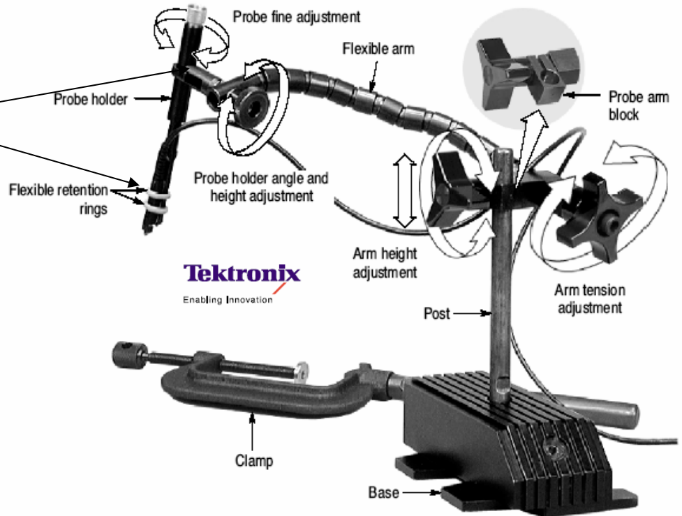
GigaProbes™ GPMMA attaches directly to the end of the Tektronix PPM203B
