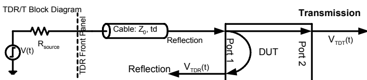
Figure 1. Time Domain Reflection and Transmission (TDR and TDT) block diagram. A similar diagram can be drawn for reverse measurements (from port 2 to port 1).
